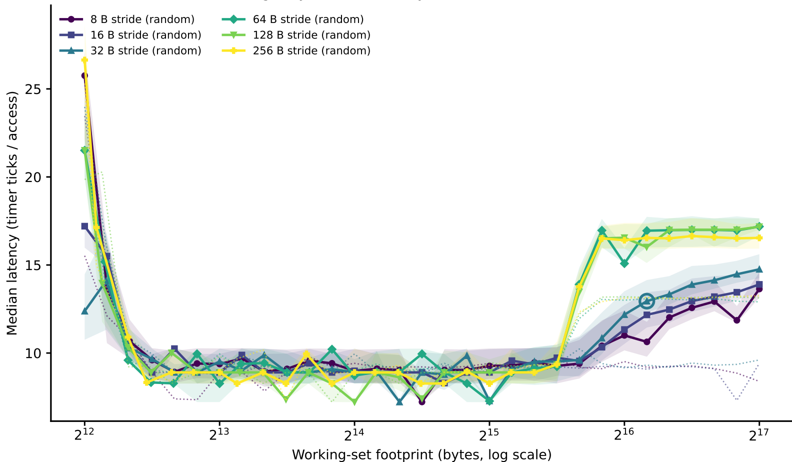
hazel_icelake_6326: line-size family of curves (dependent pointer chase) (Phase I timing-only, level boundary=32768B window=[4096,131072])
