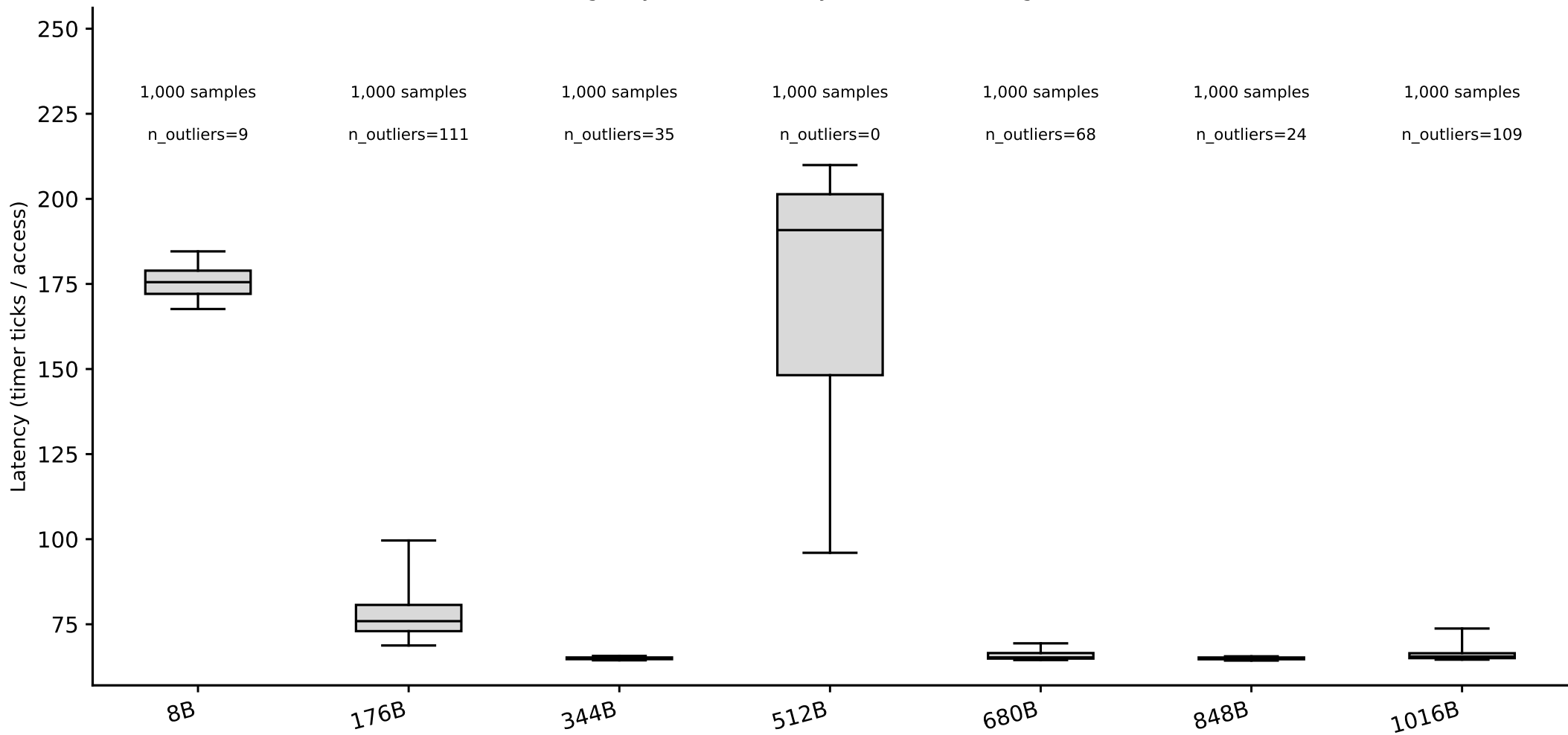
hazel_icelake_6326/line_size_rerun: line-size box plots, random pattern (whiskers = p5/p95) (Phase I timing-only, level boundary=25874000B, single-curve method)
