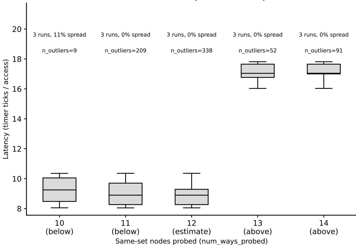
hazel_icelake_6326/phase1_v2: associativity box plots, L2, random pattern (whiskers = p5/p99) (Phase I timing-only, auto pipeline) detected associativity estimate: 12-way
