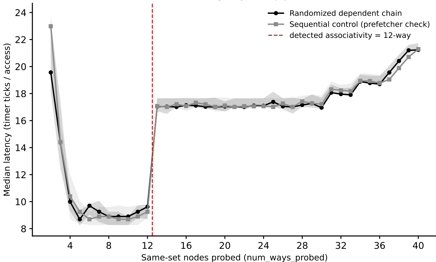
hazel_icelake_6326/phase1_v2: associativity sweep, L3_LLC (stride=24.6758 MiB) (Phase I timing-only, auto pipeline)
