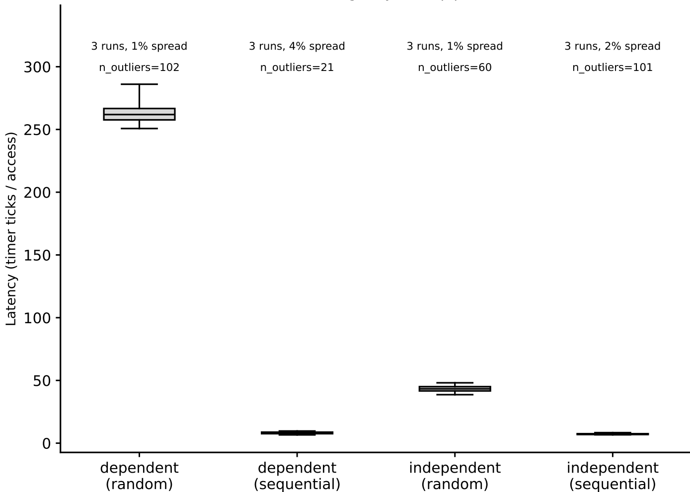
hazel_icelake_6326/phase1_v2: hit-latency box plots, DRAM (footprint=512 MiB) (Phase I timing-only, auto pipeline)
