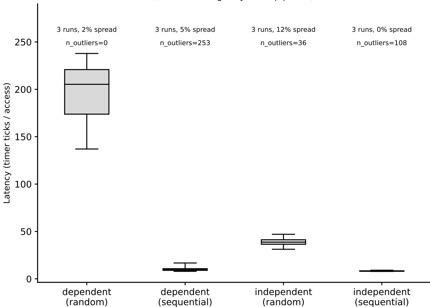
hazel_icelake_6326/phase1_v2: hit-latency box plots, LLC (footprint=24.6754 MiB) (Phase I timing-only, auto pipeline)
