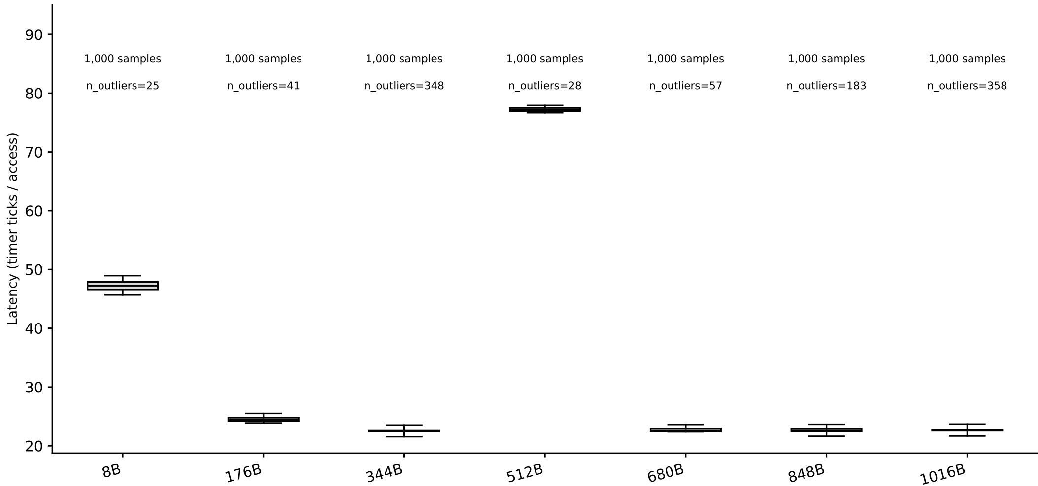
hazel_icelake_6326/phase1_v2: line-size box plots, random pattern (whiskers = p5/p95) (Phase I timing-only, level boundary=1310720B, single-curve method)
