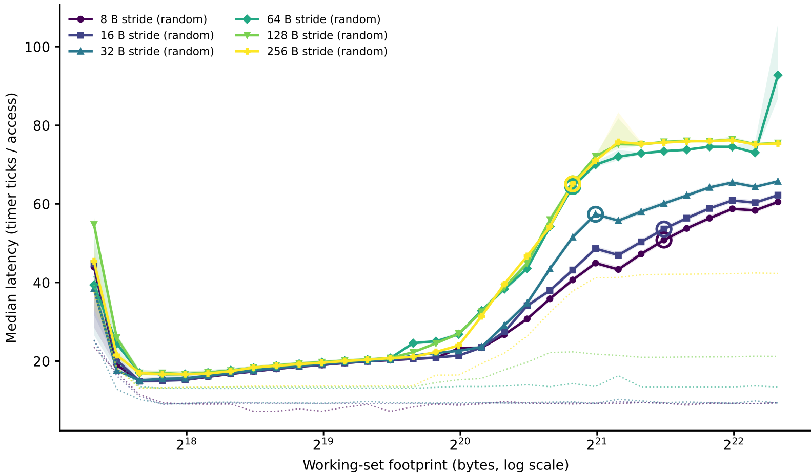
hazel_icelake_6326/phase1_v2: line-size family of curves (dependent pointer chase) (Phase I timing-only, level boundary=1310720B window=[163840,524288])
