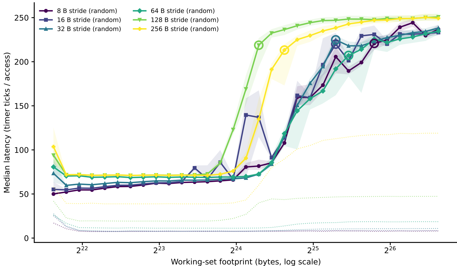
hazel_icelake_6326/phase1_v2: line-size family of curves (dependent pointer chase) (Phase I timing-only, level boundary=25874000B window=[3234250,103496000])
