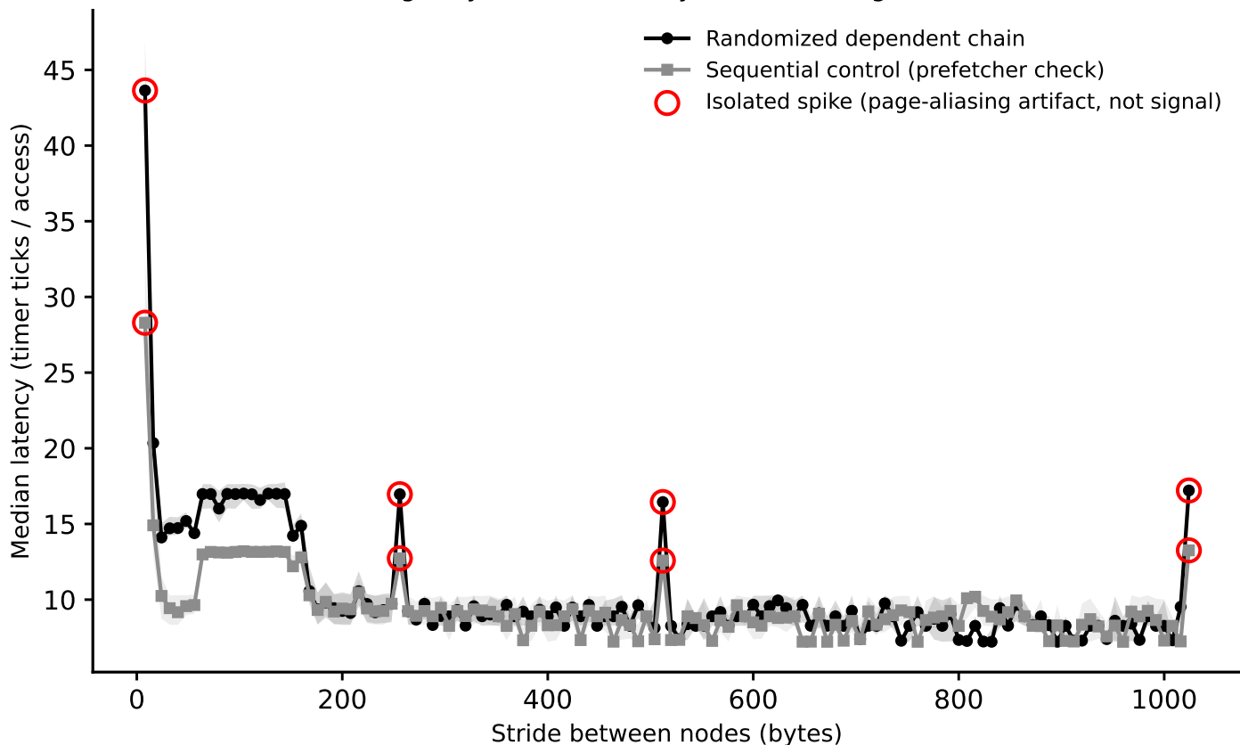
hazel_icelake_6326/phase1_v2: line-size sweep (dependent pointer chase), footprint=128 KiB (Phase I timing-only, level boundary=65536B, single-curve method)
