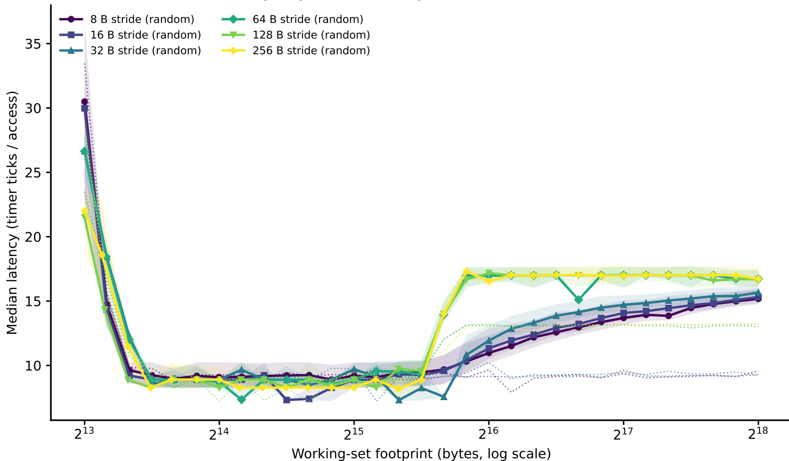
hazel_icelake_6326/phase1_v2: line-size family of curves (dependent pointer chase) (Phase I timing-only, level boundary=65536B window=[8192,262144])
