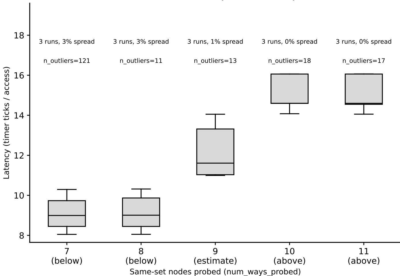
hazel_icelake_8358: associativity box plots, L1, random pattern (whiskers = p5/p95) (Phase I timing-only, auto pipeline) detected associativity estimate: 9-way
