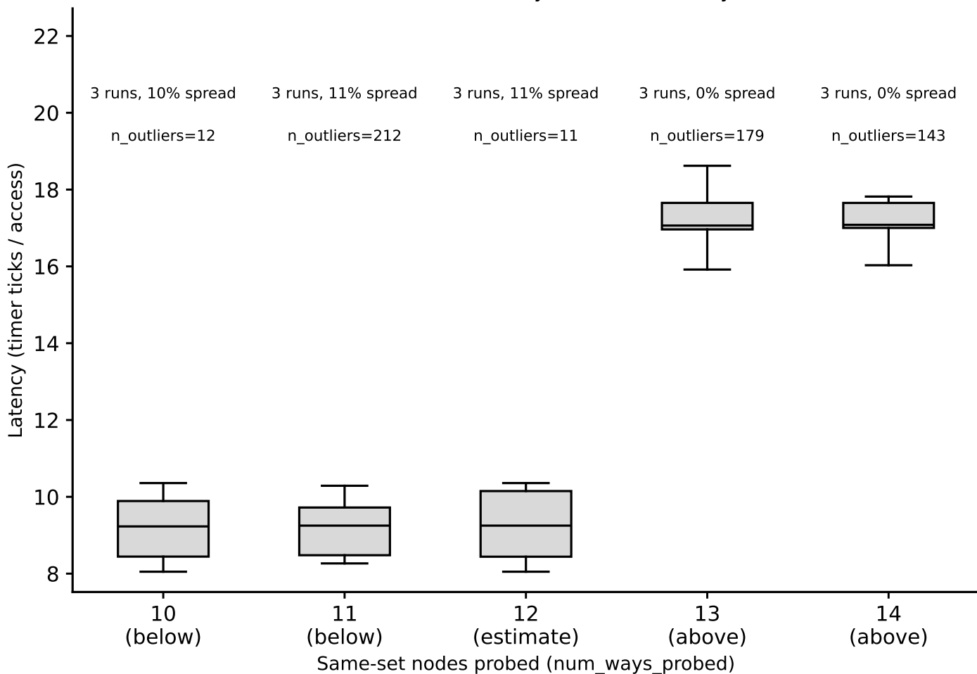
hazel_icelake_8358: associativity box plots, L2, random pattern (whiskers = p5/p95) (Phase I timing-only, auto pipeline) detected associativity estimate: 12-way
