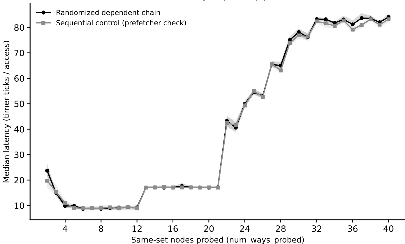
hazel_icelake_8358: associativity sweep, L2 (stride=1.25 MiB) (Phase I timing-only, auto pipeline)
