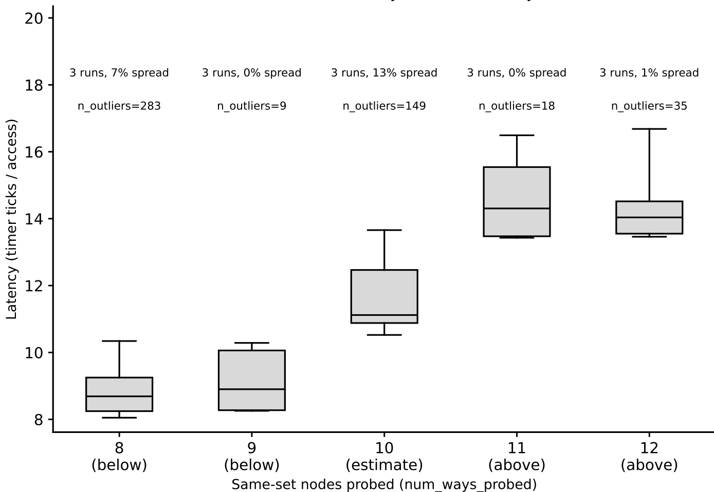
hazel_icelake_8358: associativity box plots, L3_LLC, random pattern (whiskers = p5/p95) (Phase I timing-only, auto pipeline) detected associativity estimate: 10-way
