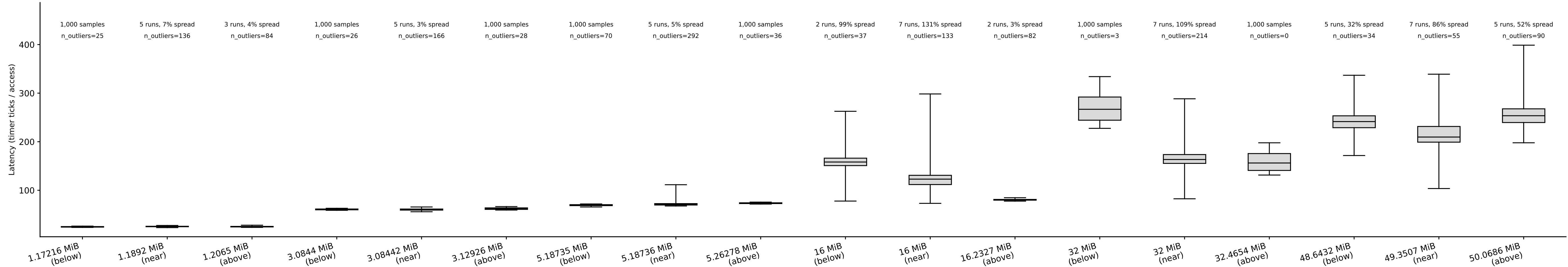
hazel_icelake_8358: capacity box plots, random pattern (whiskers = p5/p95) (Phase I timing-only, auto pipeline) tested boundaries: 1.1892 MiB, 3.08442 MiB, 5.18736 MiB, 16 MiB, 32 MiB, 49.3507 MiB
