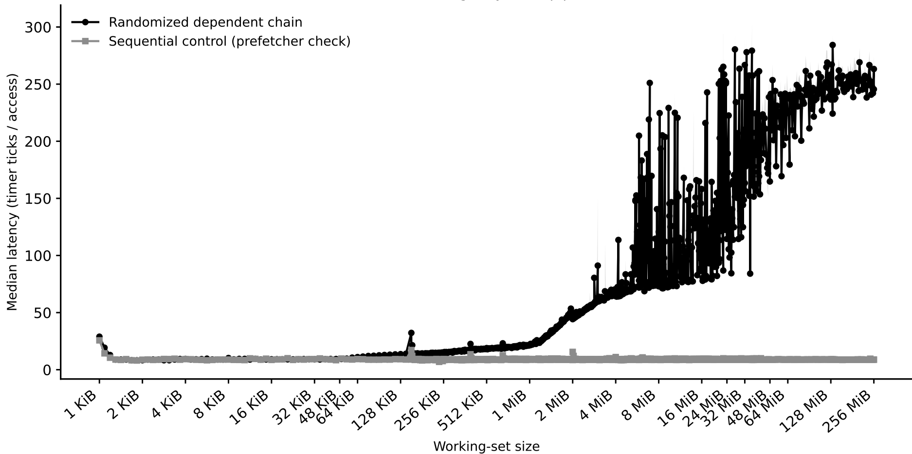
hazel_icelake_8358: capacity sweep (dependent pointer chase) (Phase I timing-only, auto pipeline)
