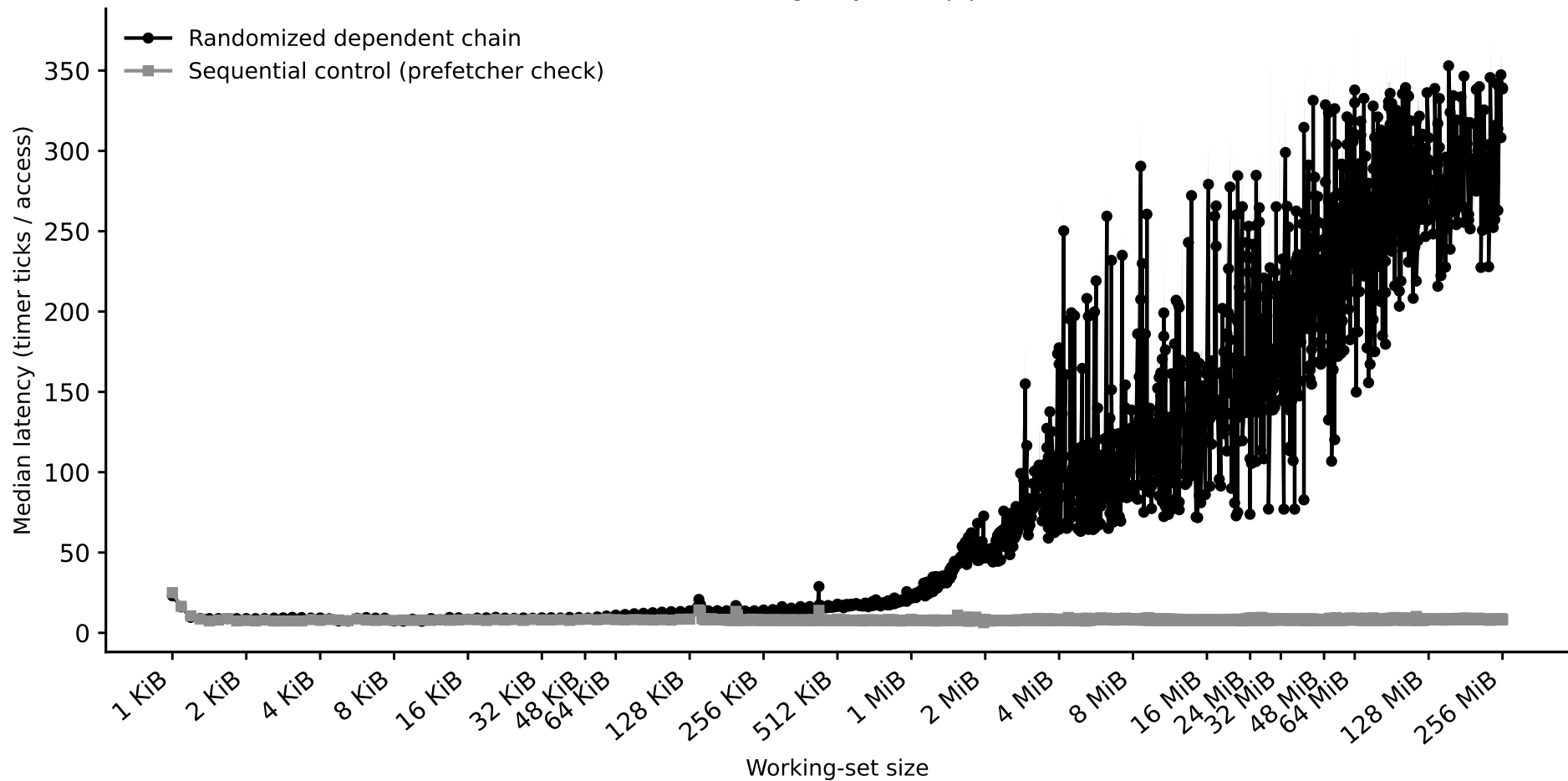
hazel_icelake_8358/capacity_rerun: capacity sweep (dependent pointer chase) (Phase I timing-only, auto pipeline)
