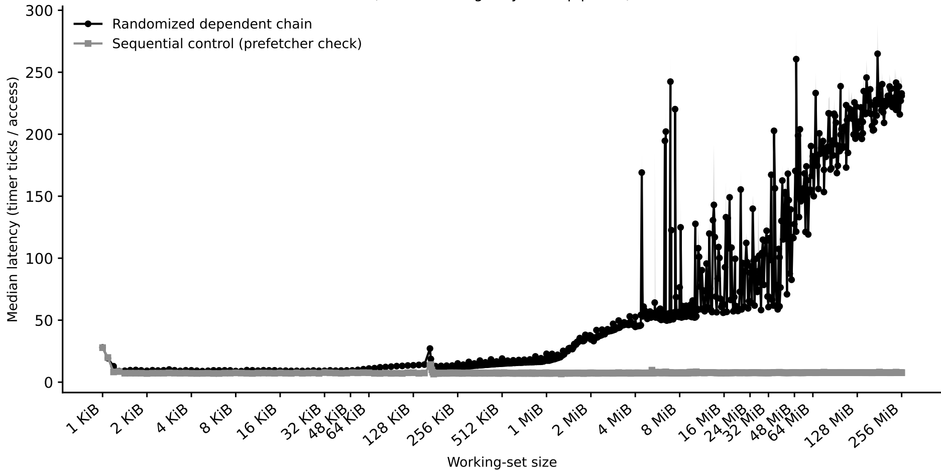
hazel_icelake_8358/capacity_rerun3: capacity sweep (dependent pointer chase) (Phase I timing-only, auto pipeline)
