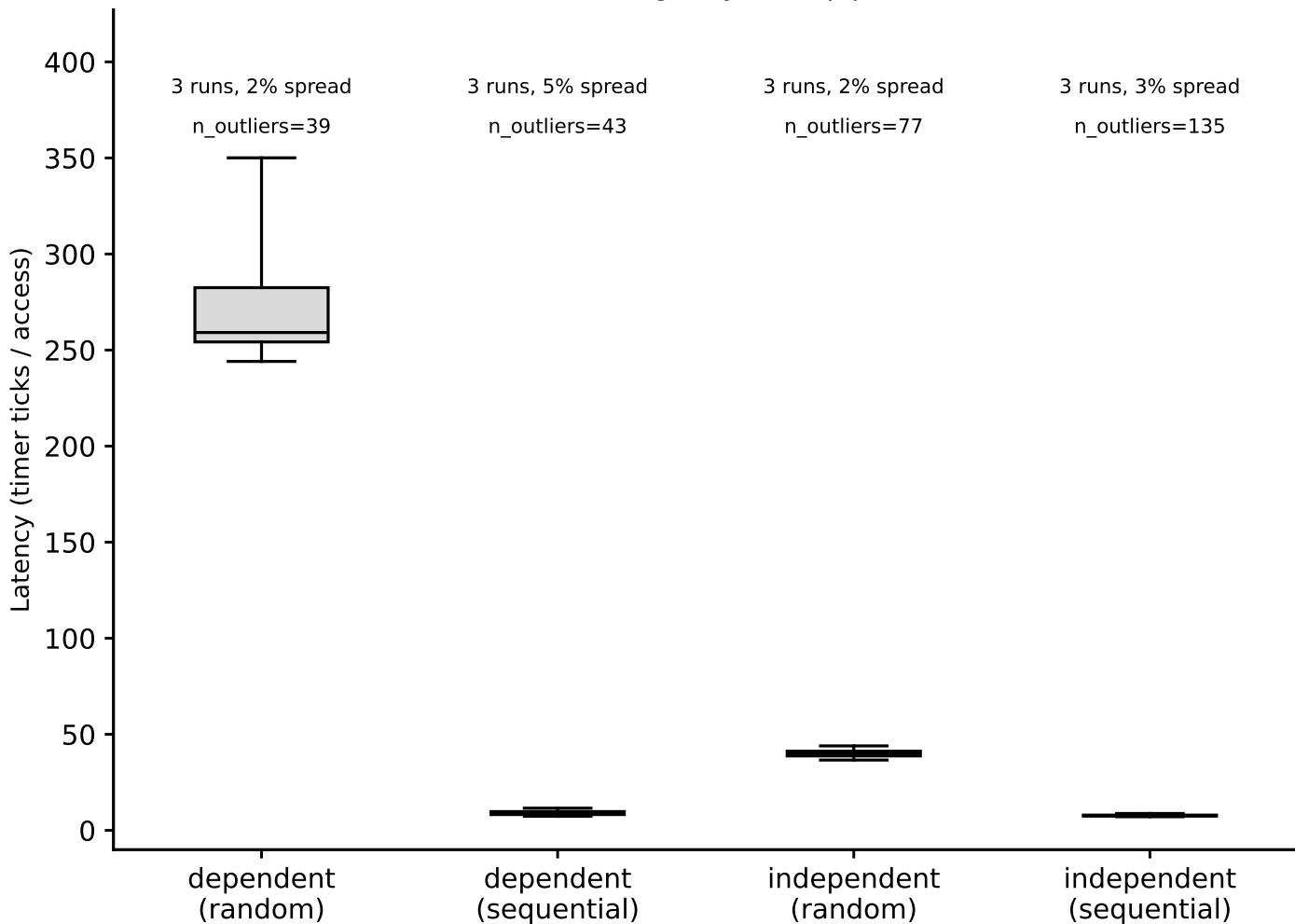
hazel_icelake_8358: hit-latency box plots, DRAM (footprint=512 MiB) (Phase I timing-only, auto pipeline)
