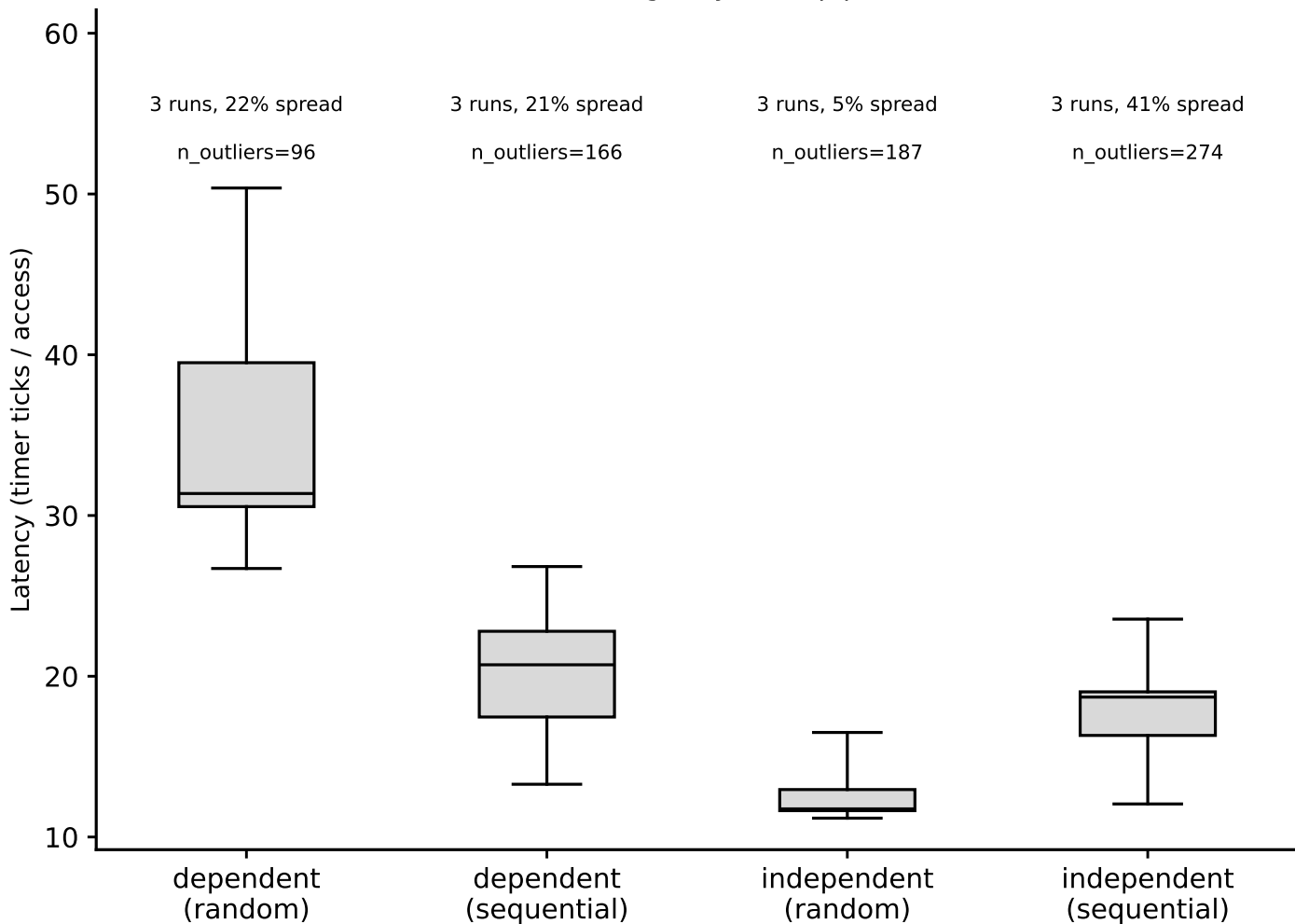
hazel_icelake_8358: hit-latency box plots, L2 (footprint=1.25 MiB) (Phase I timing-only, auto pipeline)
