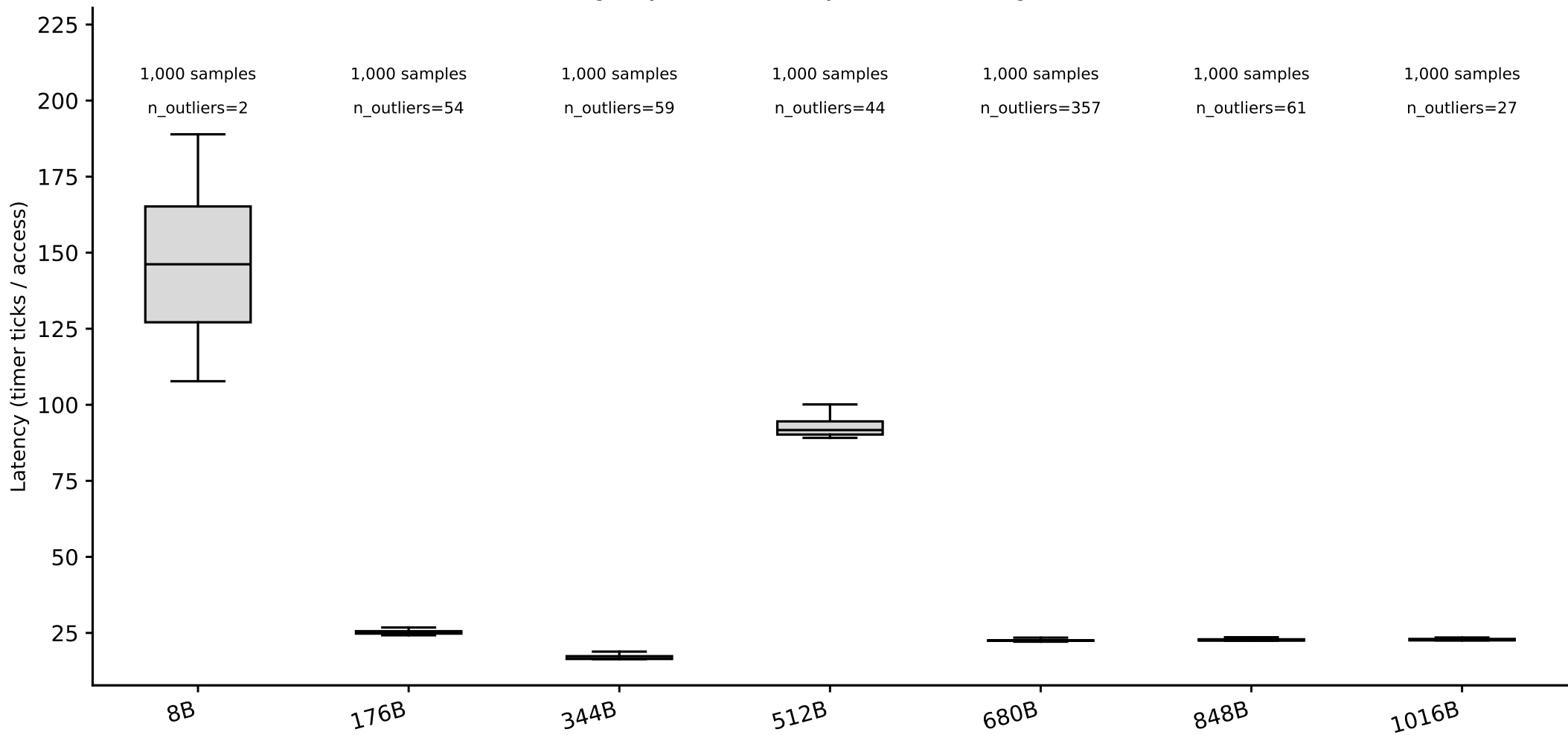
hazel_icelake_8358: line-size box plots, random pattern (whiskers = p5/p95) (Phase I timing-only, level boundary=1310720B, single-curve method)
