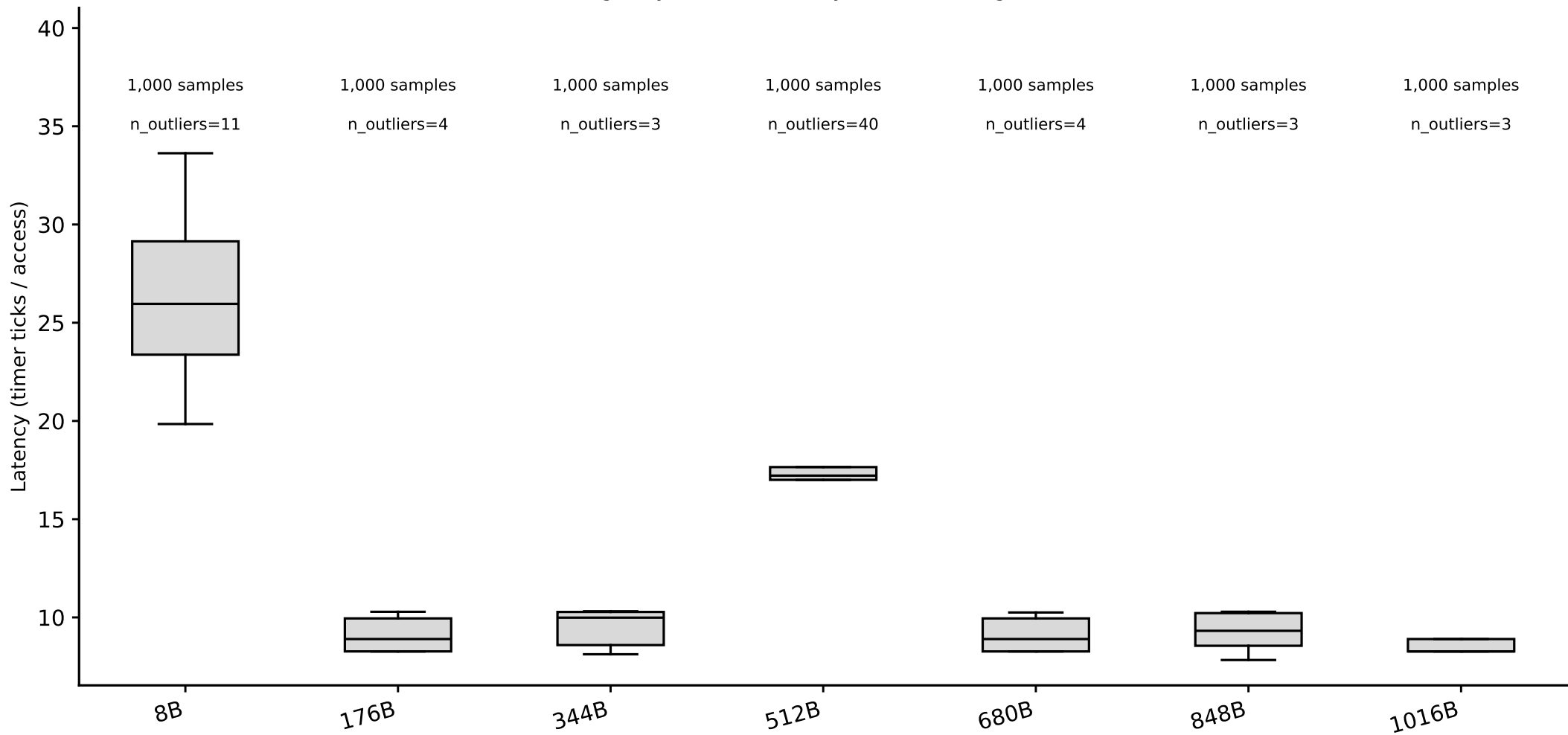
hazel_icelake_8358: line-size box plots, random pattern (whiskers = p5/p95) (Phase I timing-only, level boundary=32768B, single-curve method)
