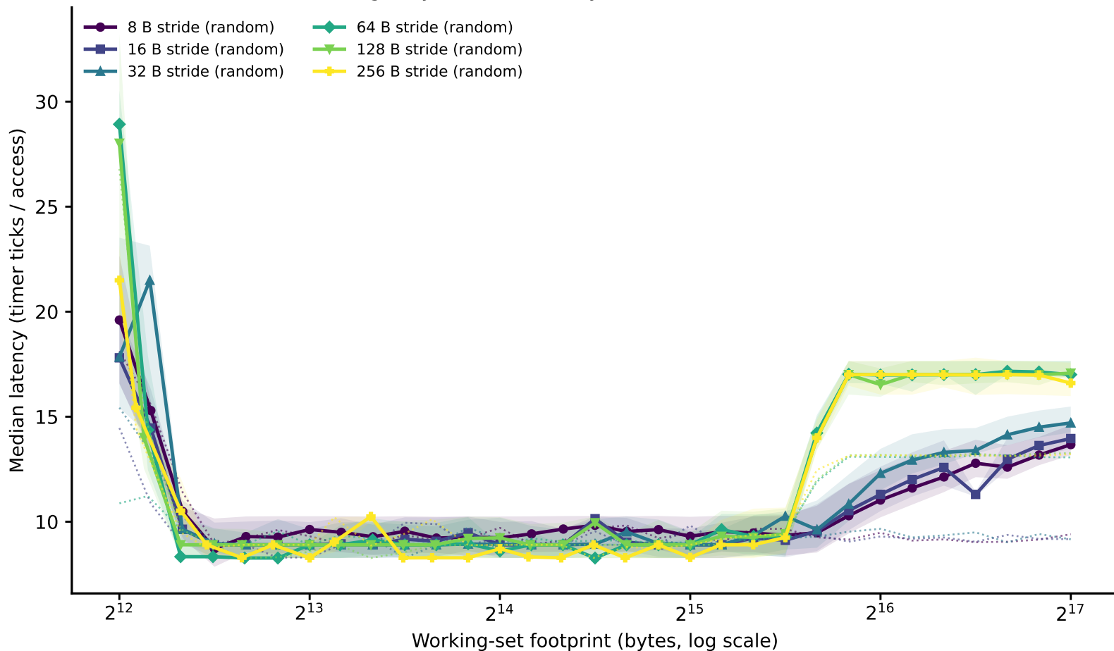
hazel_icelake_8358: line-size family of curves (dependent pointer chase) (Phase I timing-only, level boundary=32768B window=[4096,131072])
