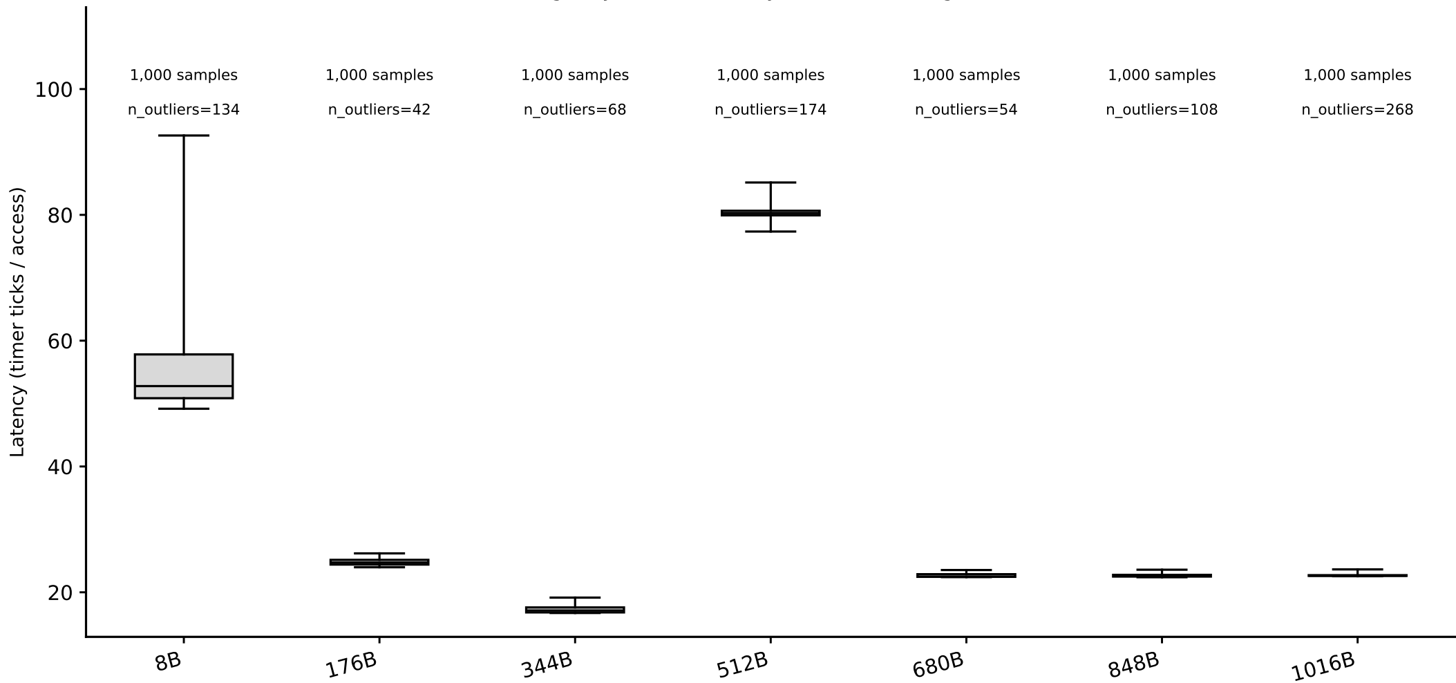
hazel_icelake_8358/line_size_rerun: line-size box plots, random pattern (whiskers = p5/p95) (Phase I timing-only, level boundary=1310720B, single-curve method)
