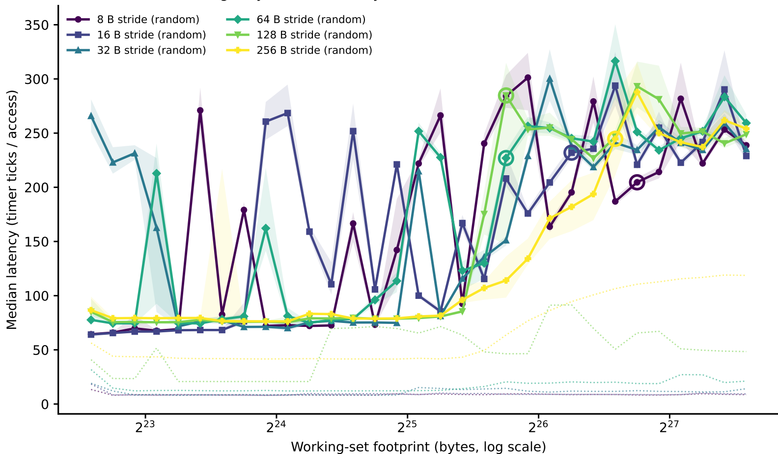
hazel_icelake_8358/line_size_rerun: line-size family of curves (dependent pointer chase) (Phase I timing-only, level boundary=50331648B window=[6291456,201326592])
