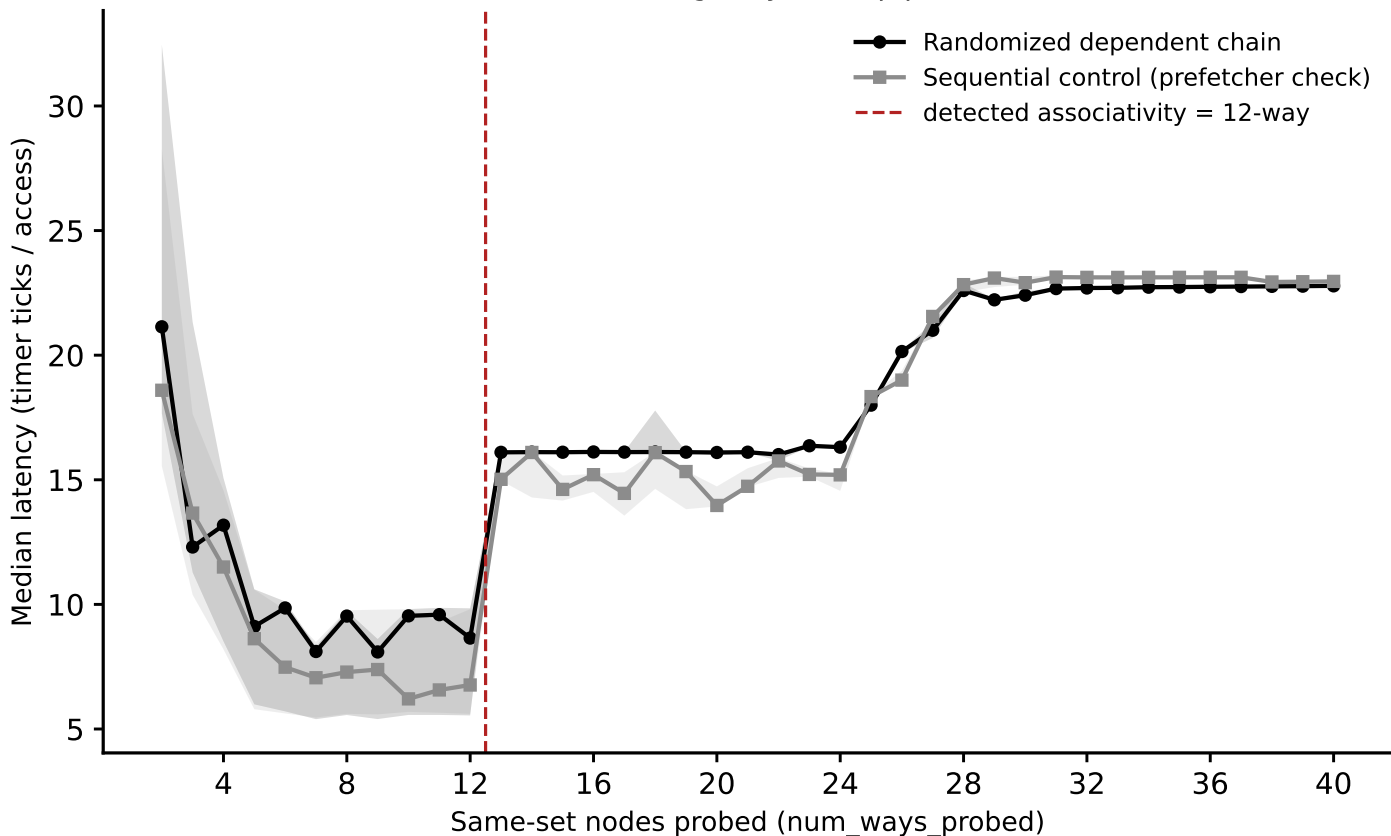
hazel_sapphirerapids: associativity sweep, L1 (stride=48 KiB) (Phase I timing-only, auto pipeline)
