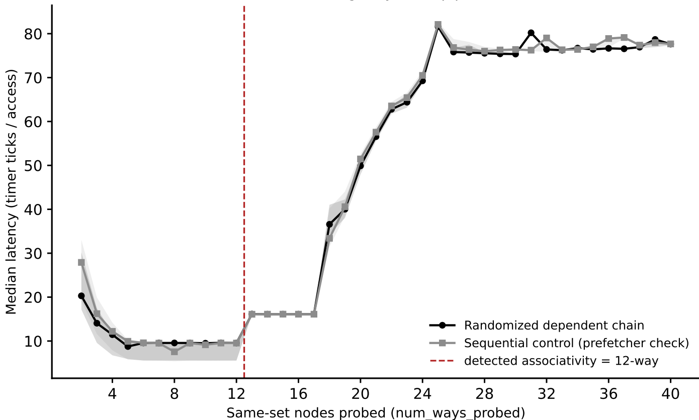
hazel_sapphirerapids: associativity sweep, L2 (stride=2 MiB) (Phase I timing-only, auto pipeline)
