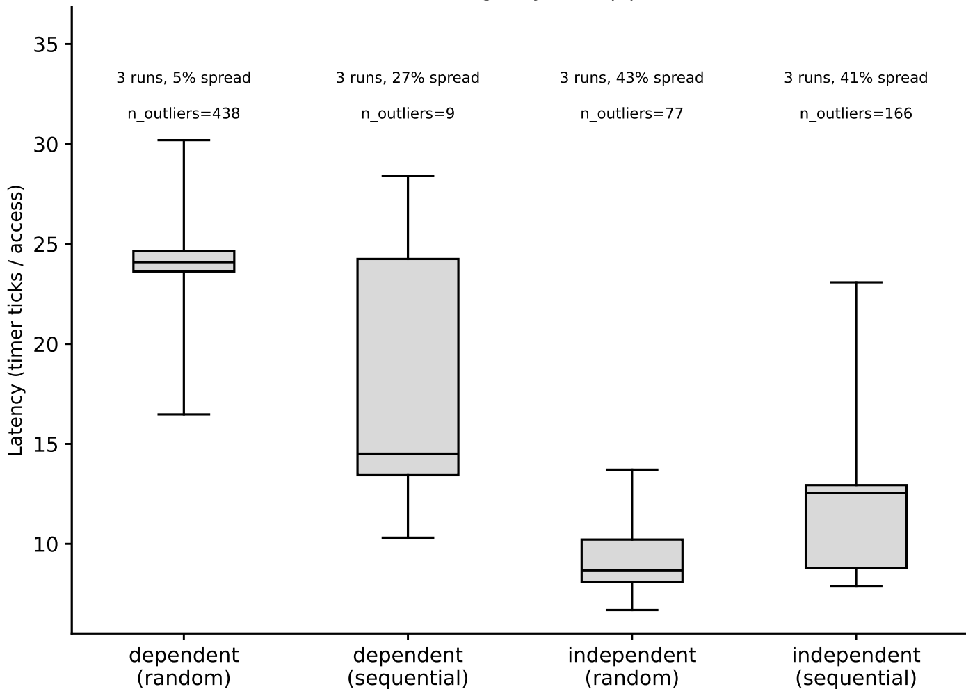
hazel_sapphirerapids: hit-latency box plots, L2 (footprint=2 MiB) (Phase I timing-only, auto pipeline)
