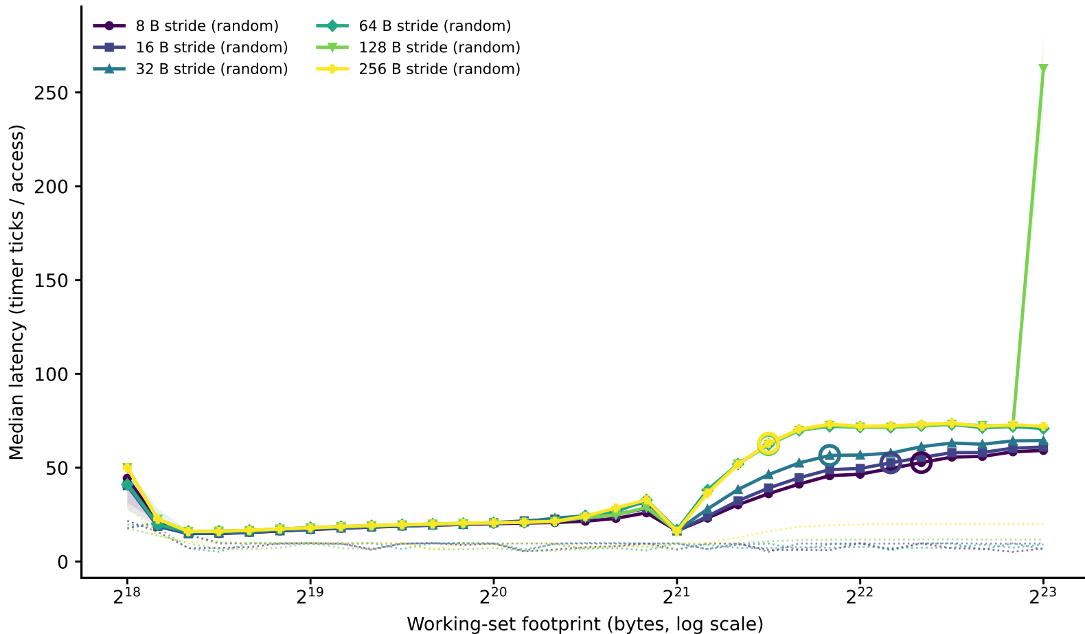
hazel_sapphirerapids: line-size family of curves (dependent pointer chase) (Phase I timing-only, level boundary=2097152B window=[262144,8388608])
