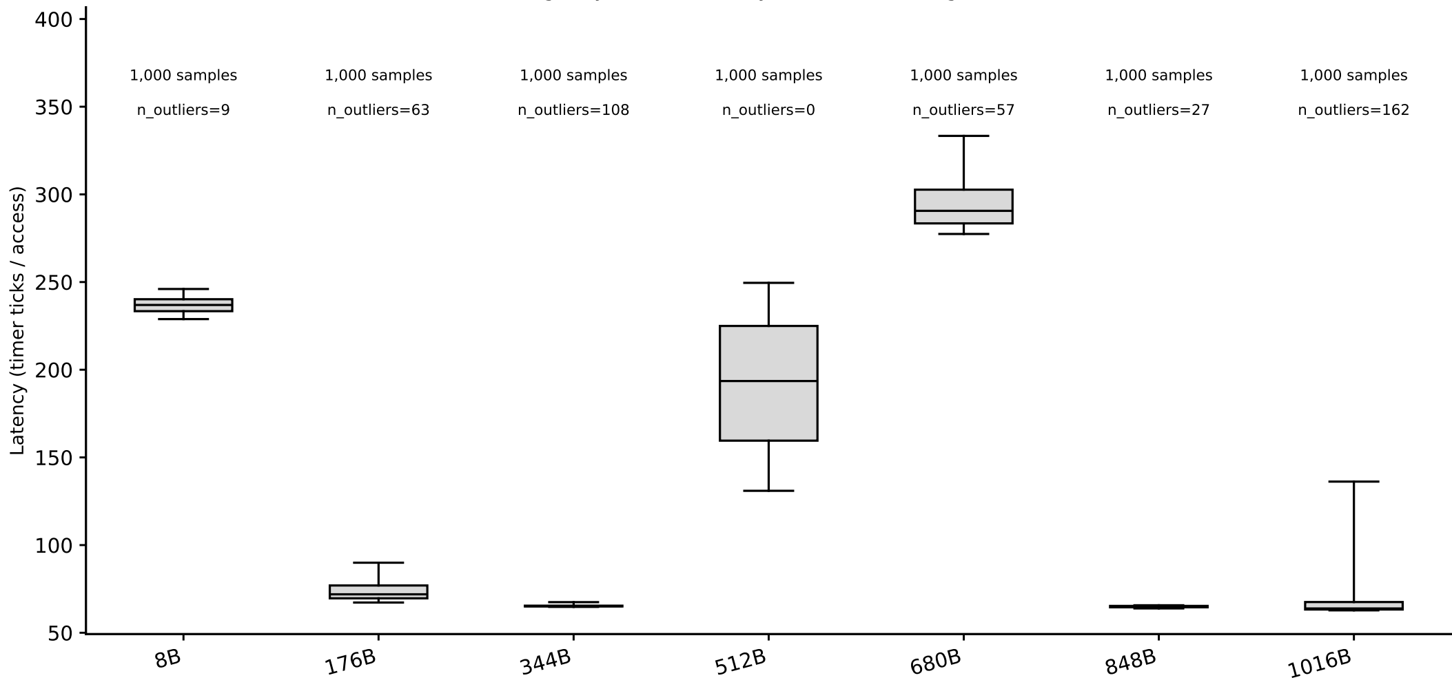
hazel_sapphirerapids: line-size box plots, random pattern (whiskers = p5/p95) (Phase I timing-only, level boundary=39903168B, single-curve method)
