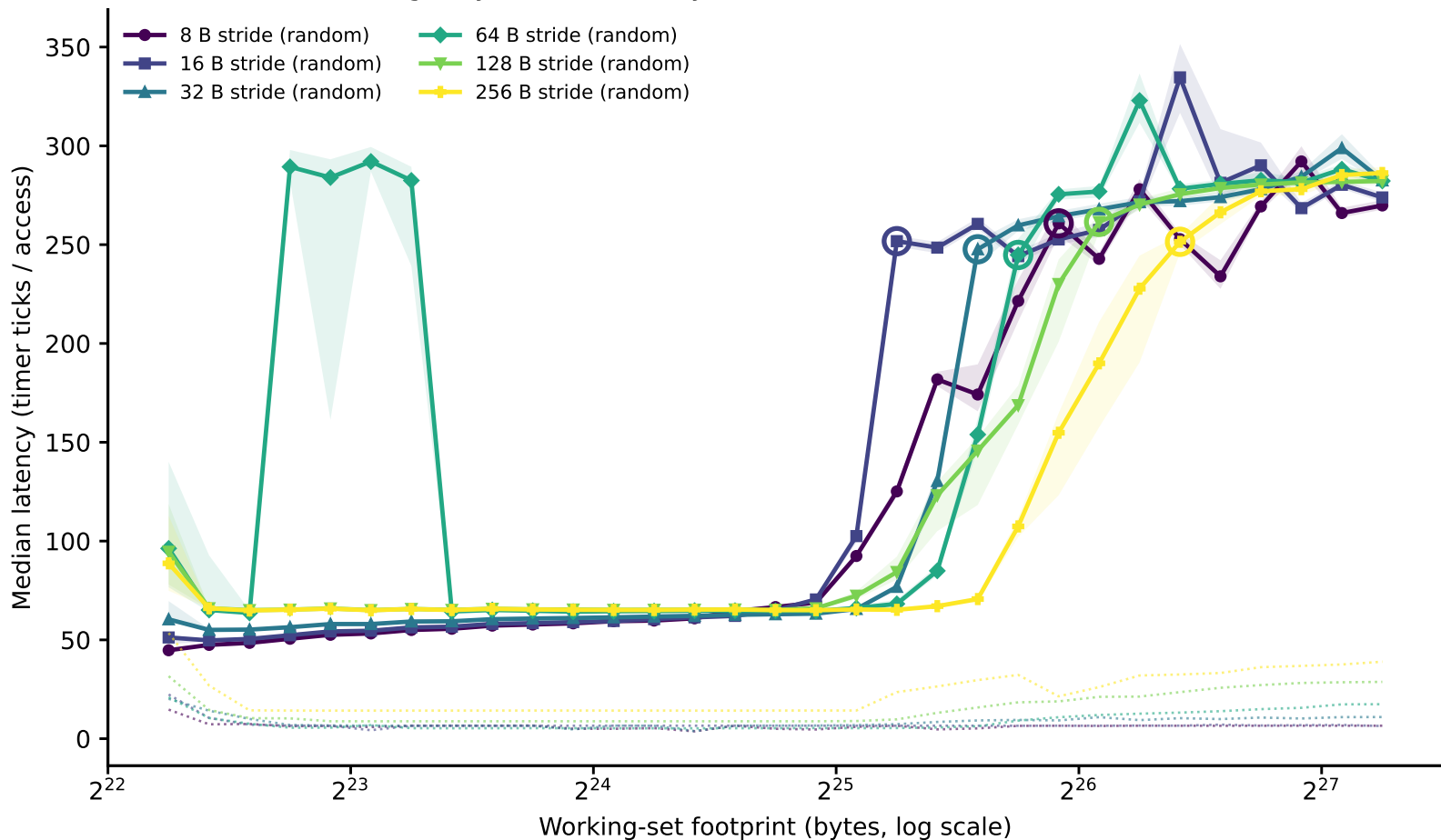
hazel_sapphirerapids: line-size family of curves (dependent pointer chase) (Phase I timing-only, level boundary=39903168B window=[4987896,159612672])
