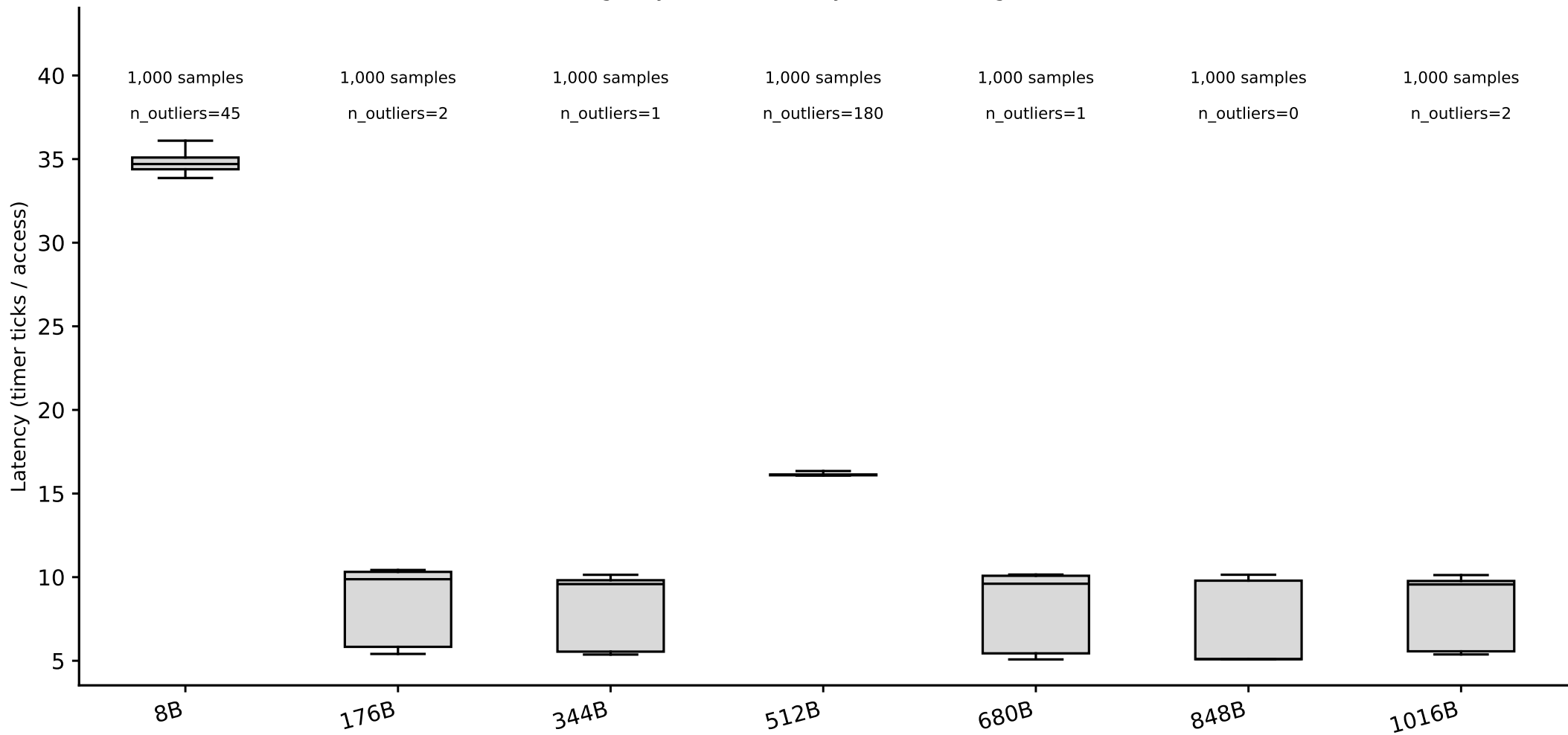
hazel_sapphirerapids: line-size box plots, random pattern (whiskers = p5/p95) (Phase I timing-only, level boundary=49152B, single-curve method)
