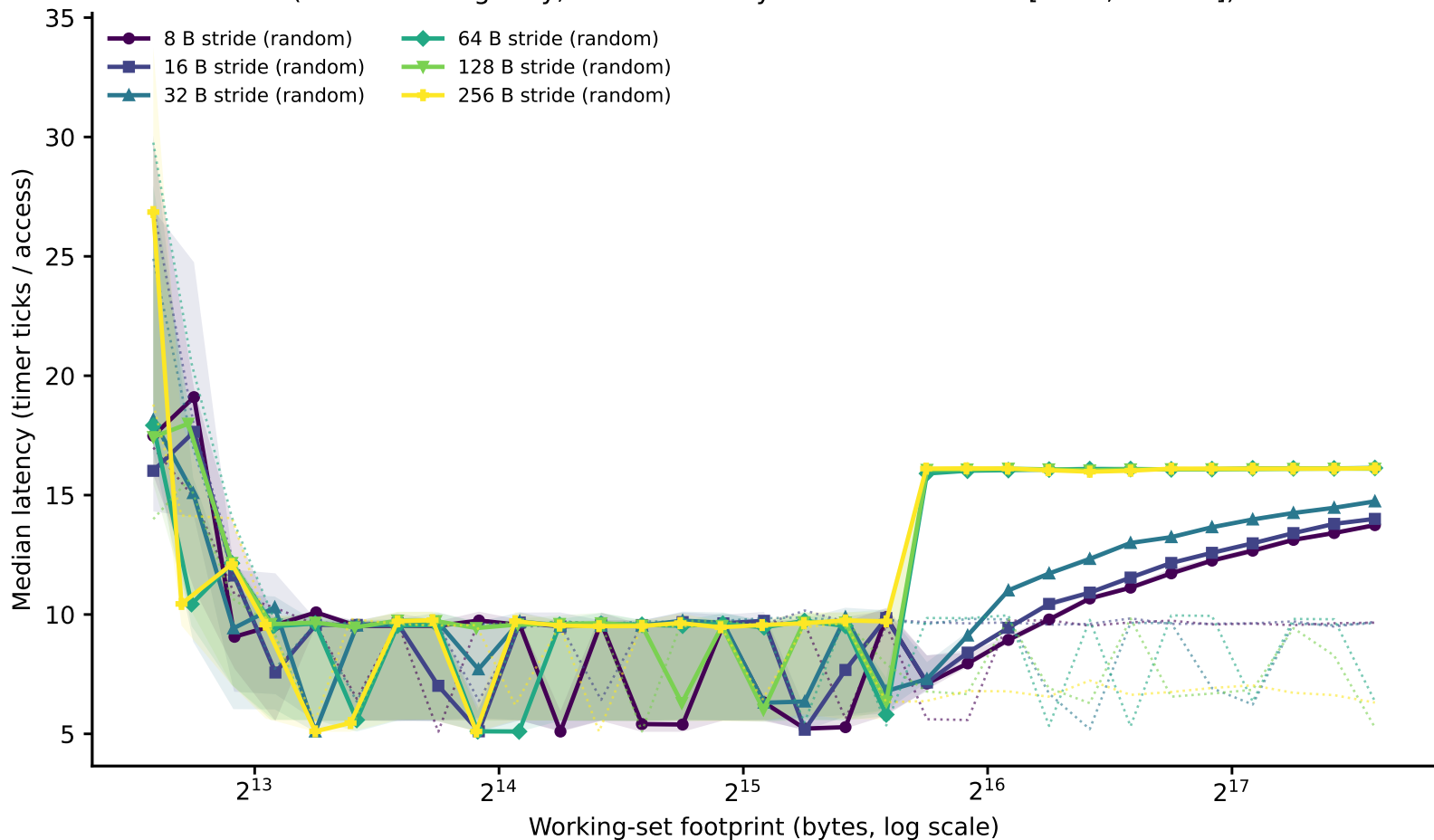
hazel_sapphirerapids: line-size family of curves (dependent pointer chase) (Phase I timing-only, level boundary=49152B window=[6144,196608])
