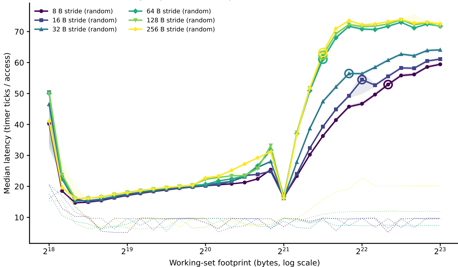
hazel_sapphirerapids/line_size_rerun: line-size family of curves (dependent pointer chase) (Phase I timing-only, level boundary=2097152B window=[262144,8388608])
