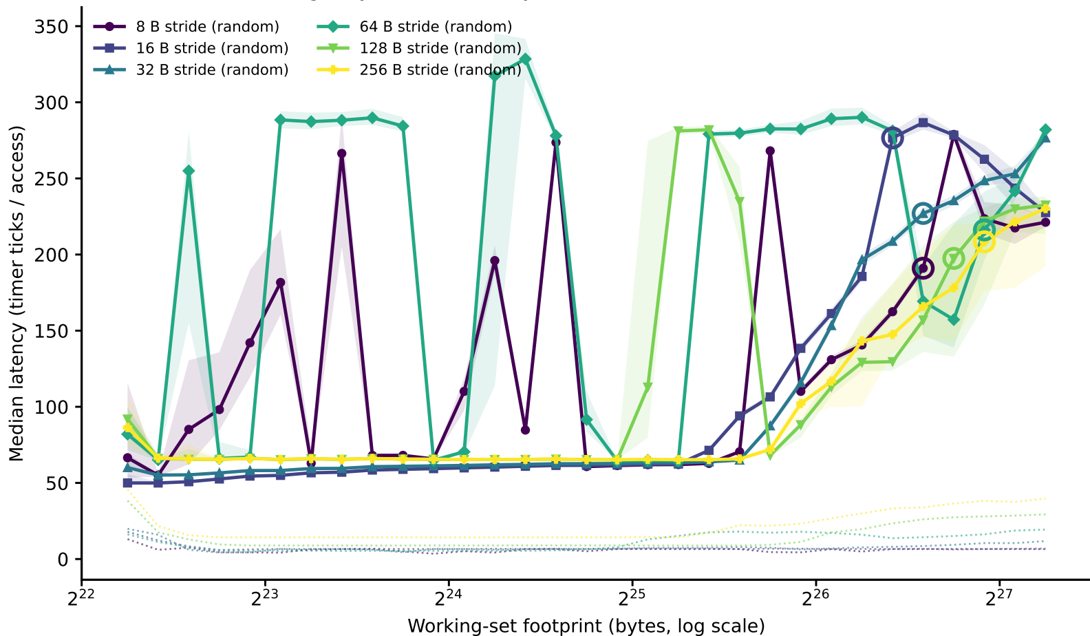
hazel_sapphirerapids/line_size_rerun: line-size family of curves (dependent pointer chase) (Phase I timing-only, level boundary=39903168B window=[4987896,159612672])
