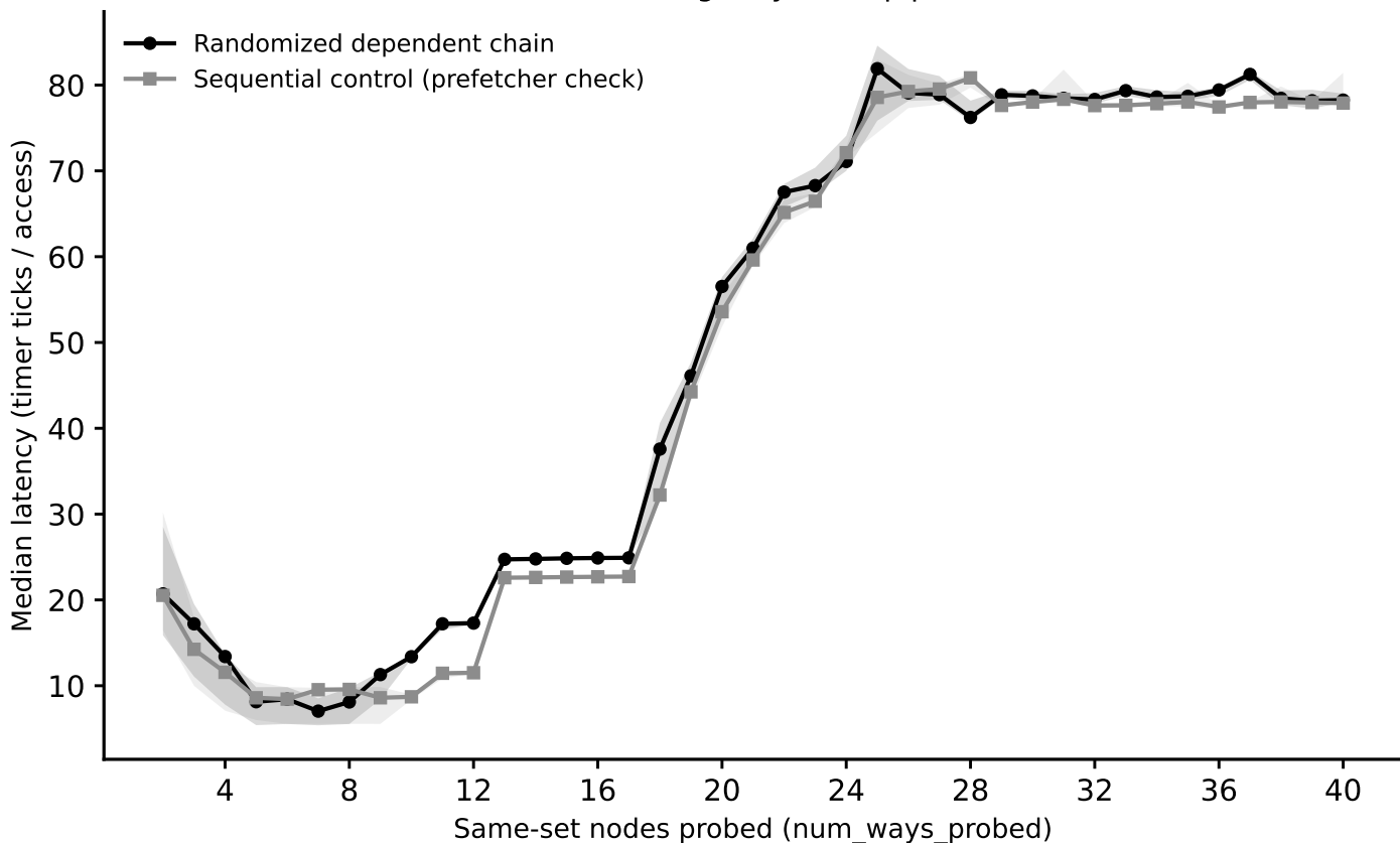
hazel_sapphirerapids/phase1_v2: associativity sweep, L3_LLC (stride=48 MiB) (Phase I timing-only, auto pipeline)
