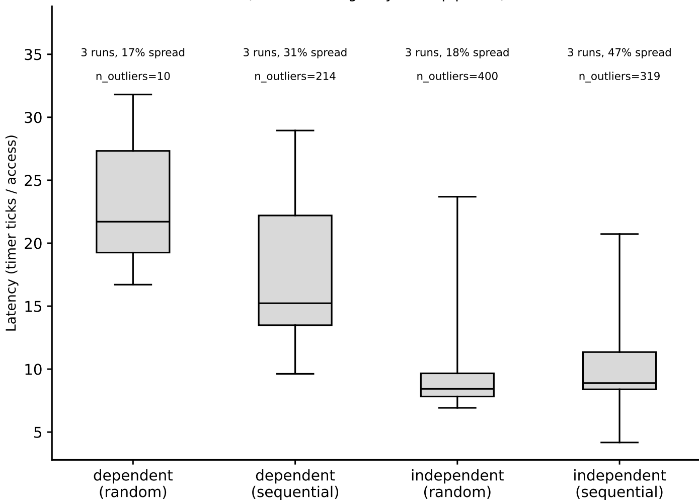
hazel_sapphirerapids/phase1_v2: hit-latency box plots, L2 (footprint=2 MiB) (Phase I timing-only, auto pipeline)
