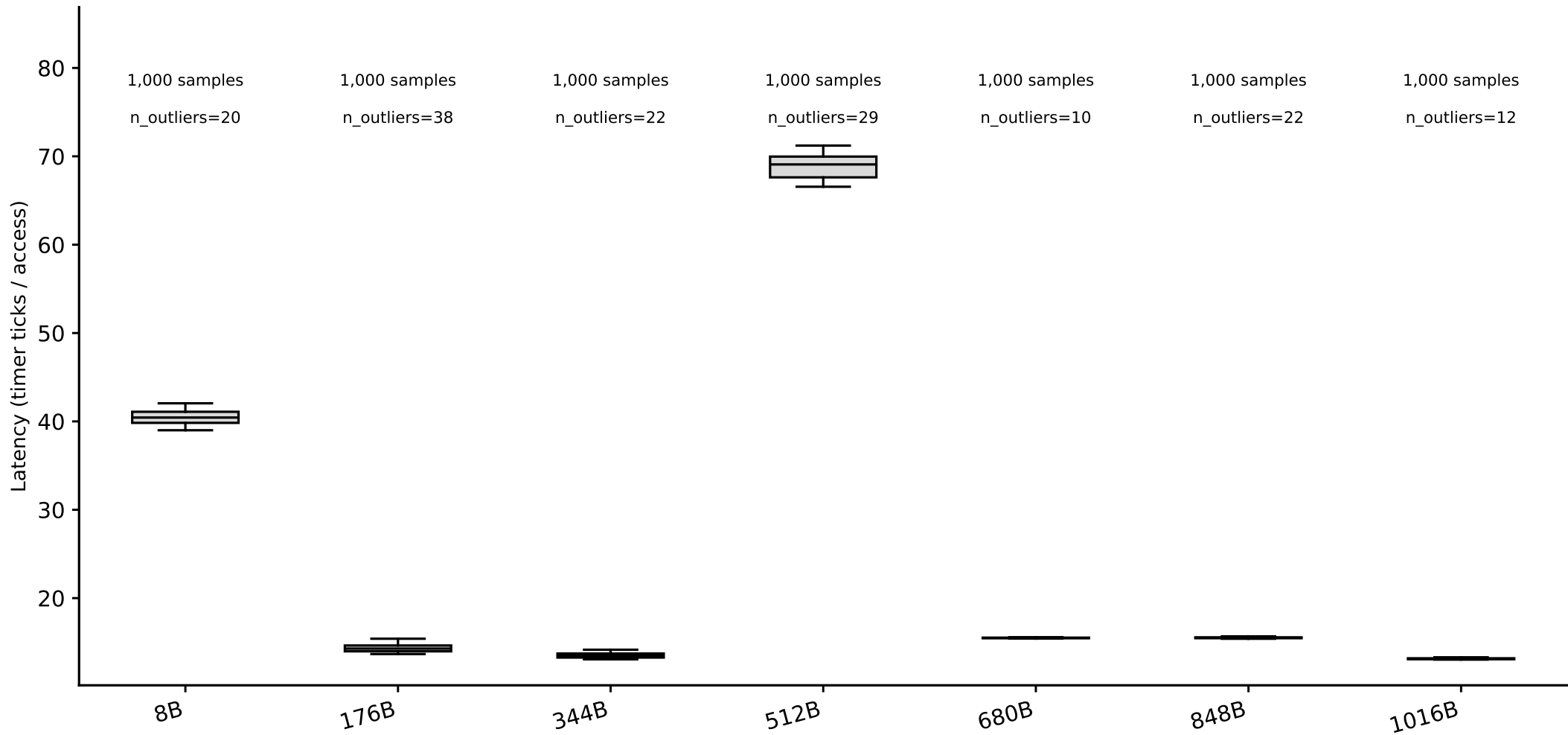
hazel_sapphirerapids/phase1_v2: line-size box plots, random pattern (whiskers = p5/p95) (Phase I timing-only, level boundary=2097152B, single-curve method)
