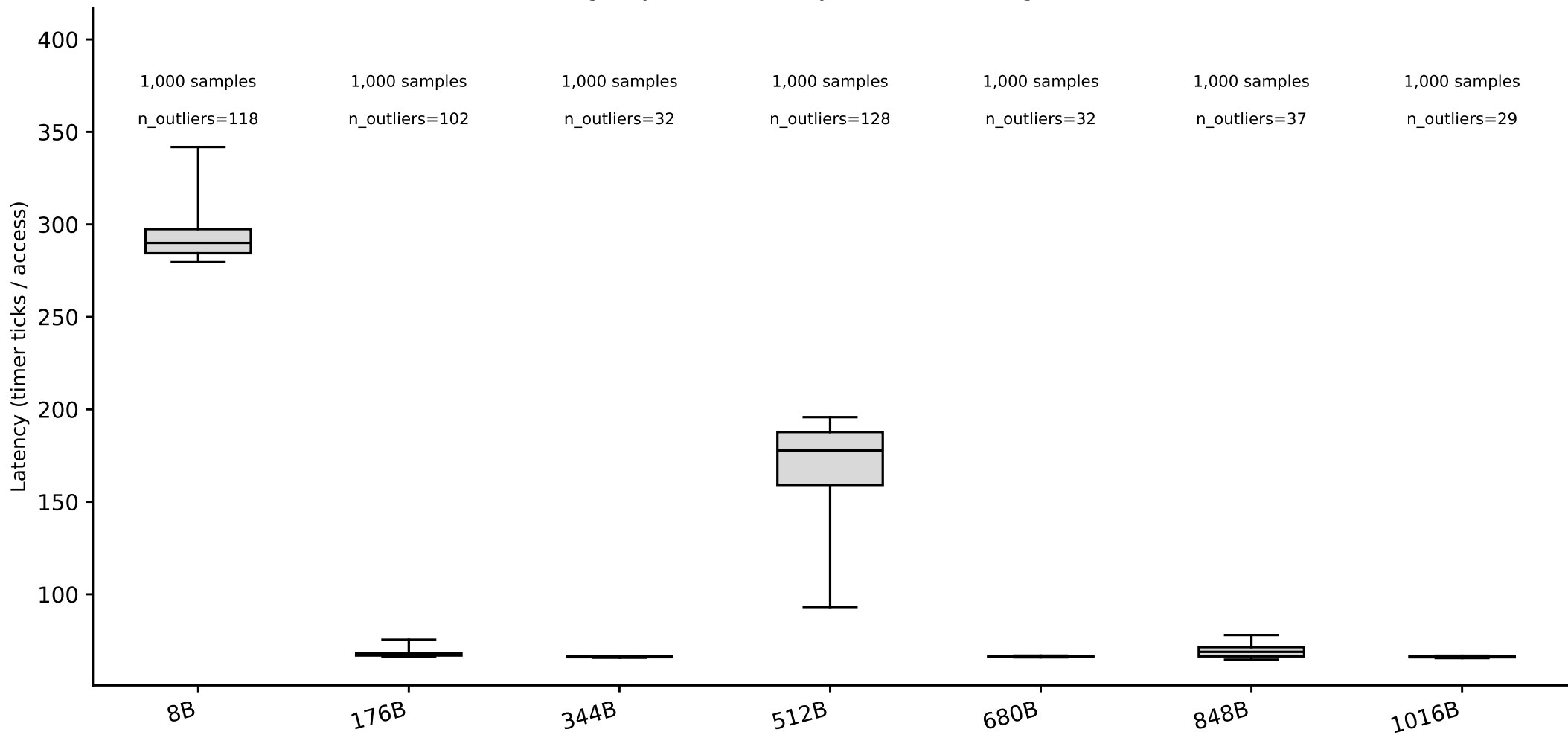
hazel_sapphirerapids/phase1_v2: line-size box plots, random pattern (whiskers = p5/p95) (Phase I timing-only, level boundary=50331648B, single-curve method)
