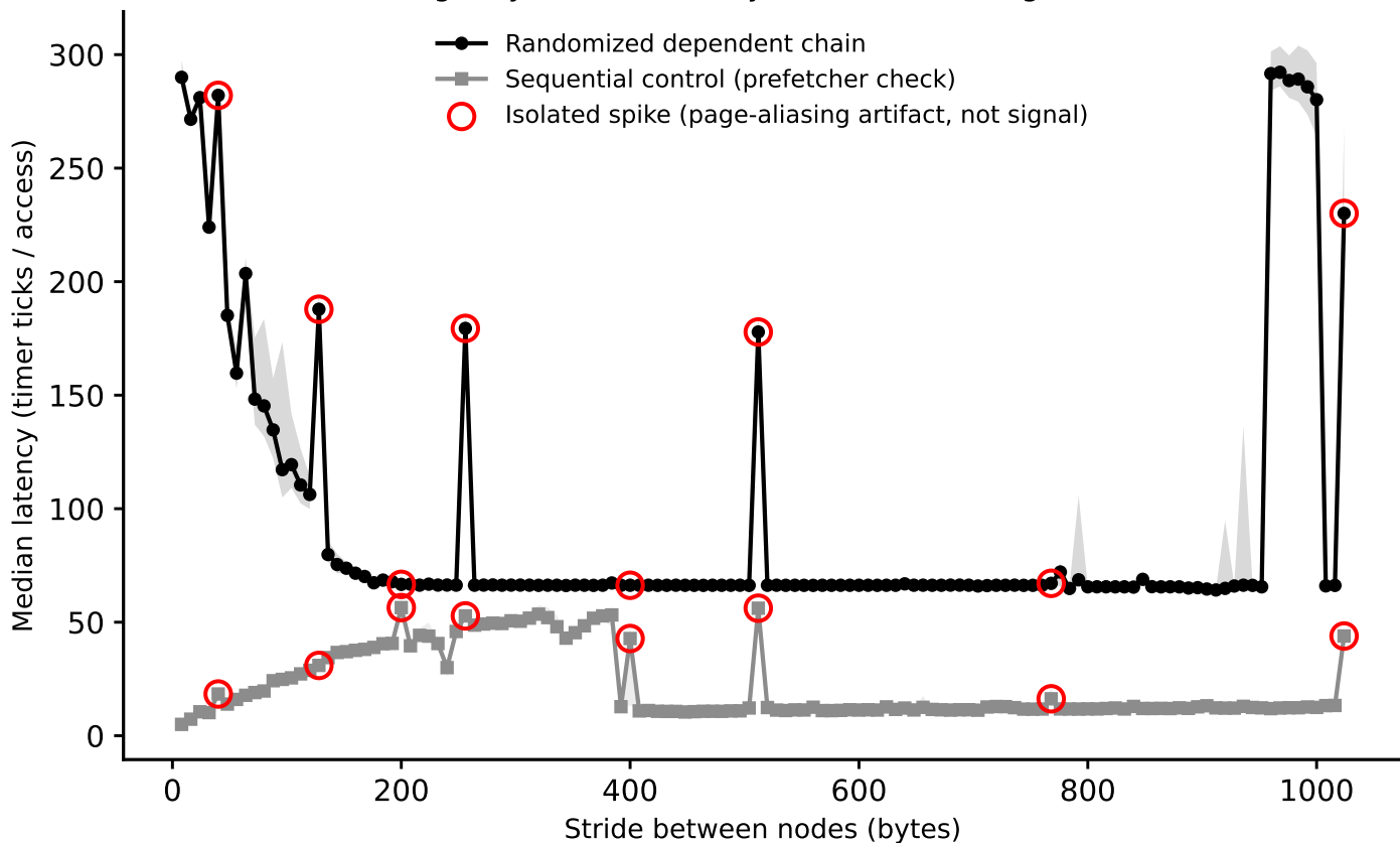
hazel_sapphirerapids/phase1_v2: line-size sweep (dependent pointer chase), footprint=96 M (Phase I timing-only, level boundary=50331648B, single-curve method)
