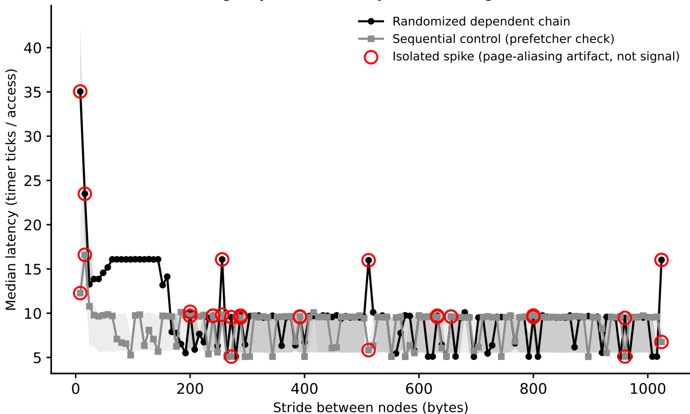
hazel_sapphirerapids/phase1_v2: line-size sweep (dependent pointer chase), footprint=128 K (Phase I timing-only, level boundary=65536B, single-curve method)
