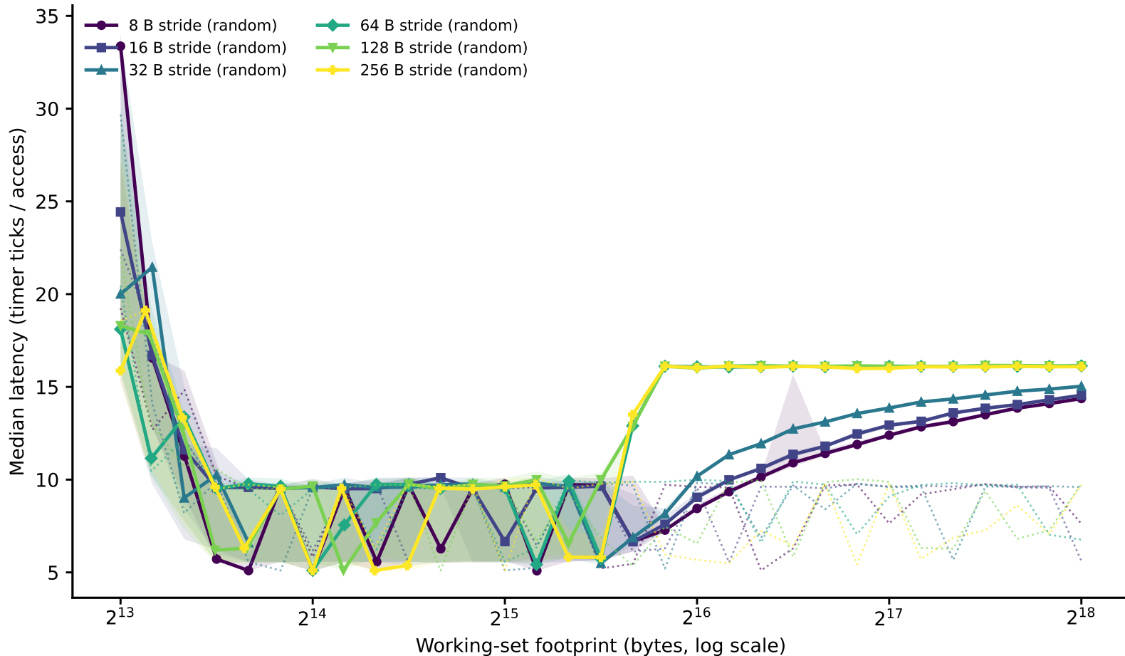
hazel_sapphirerapids/phase1_v2: line-size family of curves (dependent pointer chase) (Phase I timing-only, level boundary=65536B window=[8192,262144])
