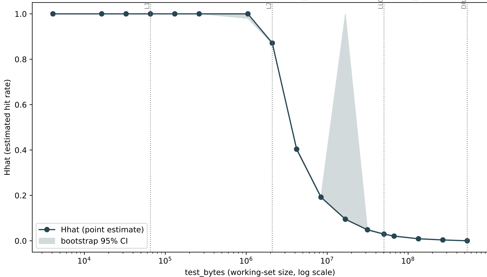
Software-only Hhat vs. working-set size (hazel_sapphirerapids/phase1_v2)
