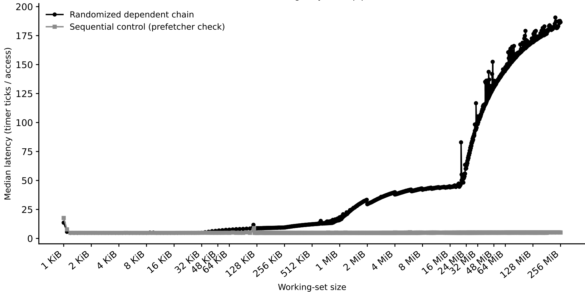
hazel_skylake/capacity_rerun: capacity sweep (dependent pointer chase) (Phase I timing-only, auto pipeline)
