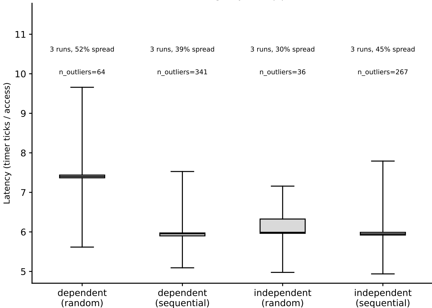
hazel_skylake: hit-latency box plots, L1 (footprint=32 KiB) (Phase I timing-only, auto pipeline)
