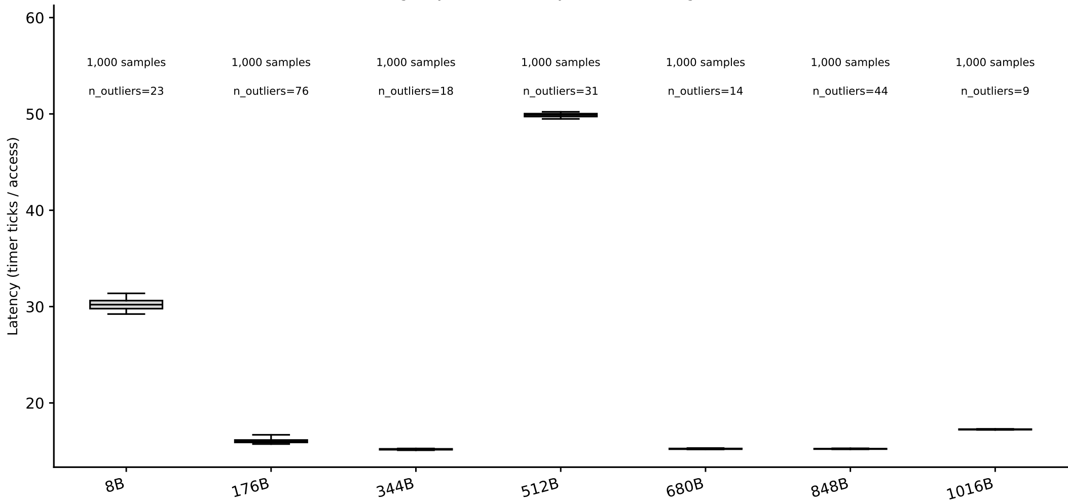
hazel_skylake: line-size box plots, random pattern (whiskers = p5/p95) (Phase I timing-only, level boundary=1048576B, single-curve method)
