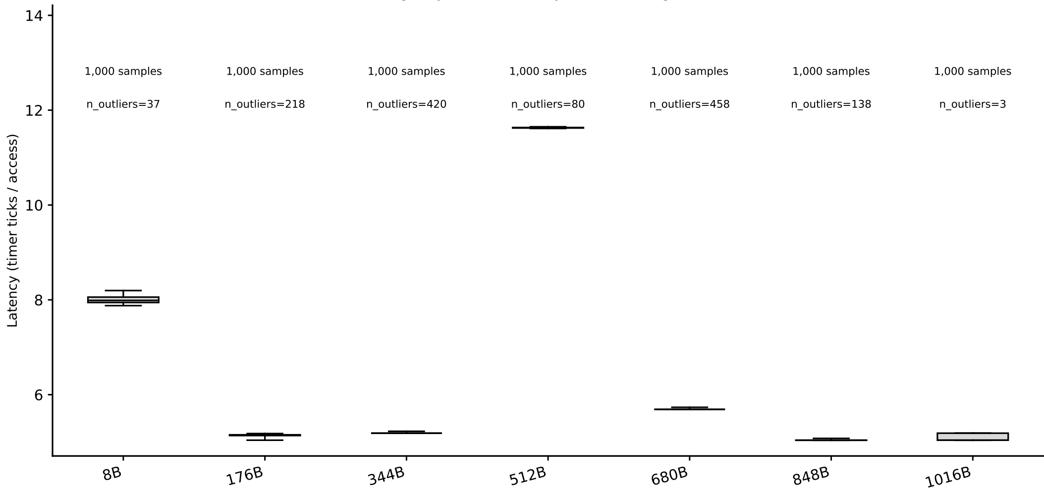
hazel_skylake: line-size box plots, random pattern (whiskers = p5/p95) (Phase I timing-only, level boundary=32768B, single-curve method)
