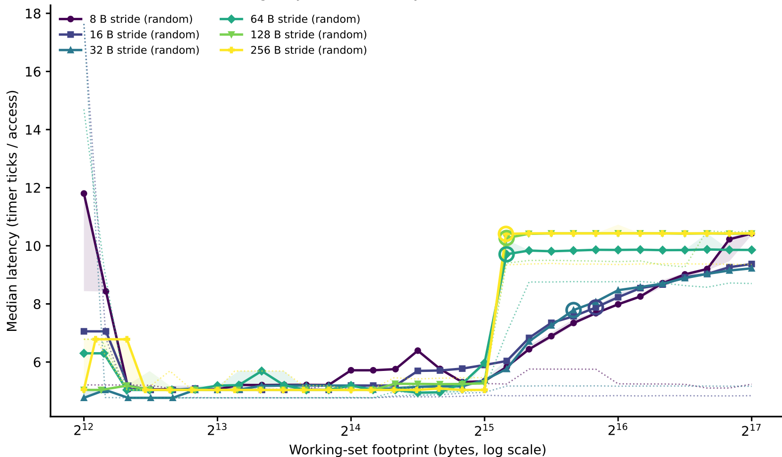
hazel_skylake: line-size family of curves (dependent pointer chase) (Phase I timing-only, level boundary=32768B window=[4096,131072])
