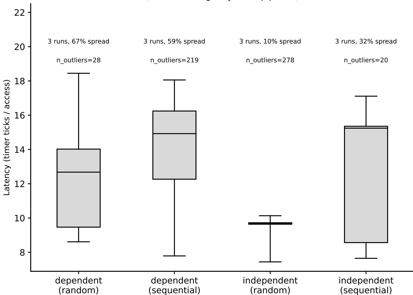
hazel_skylake/phase1_v2: hit-latency box plots, L1 (footprint=32 KiB) (Phase I timing-only, auto pipeline)
